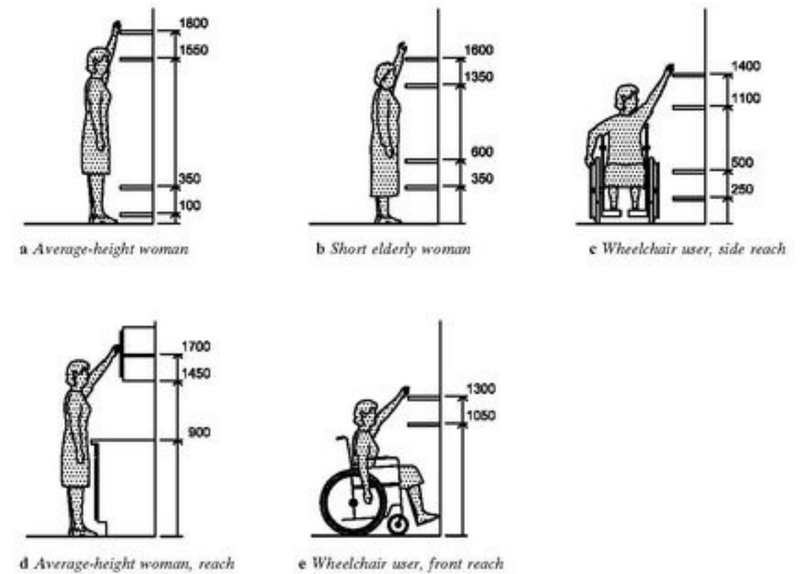
4.17 Reaches to shelves
